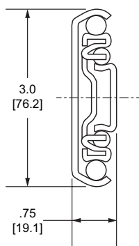
9301E/9307E/9308E Up to 600 lbs./pr. [272 kg]* * depending on usage
